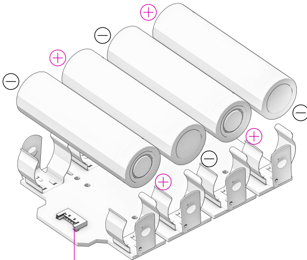
Battery Pack Cable Connector
